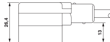
Valve connector, type BI, side view
